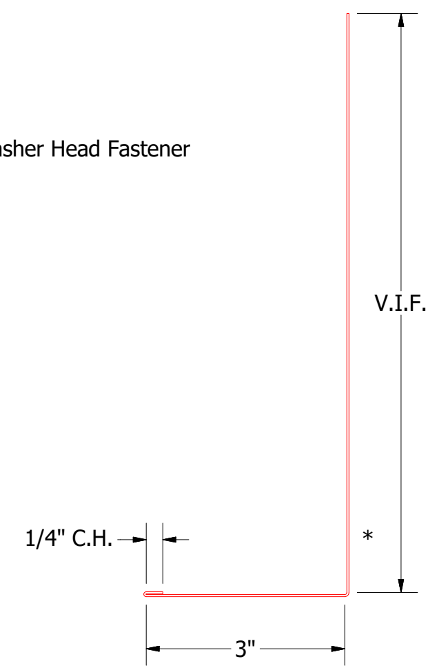
End Flashing
