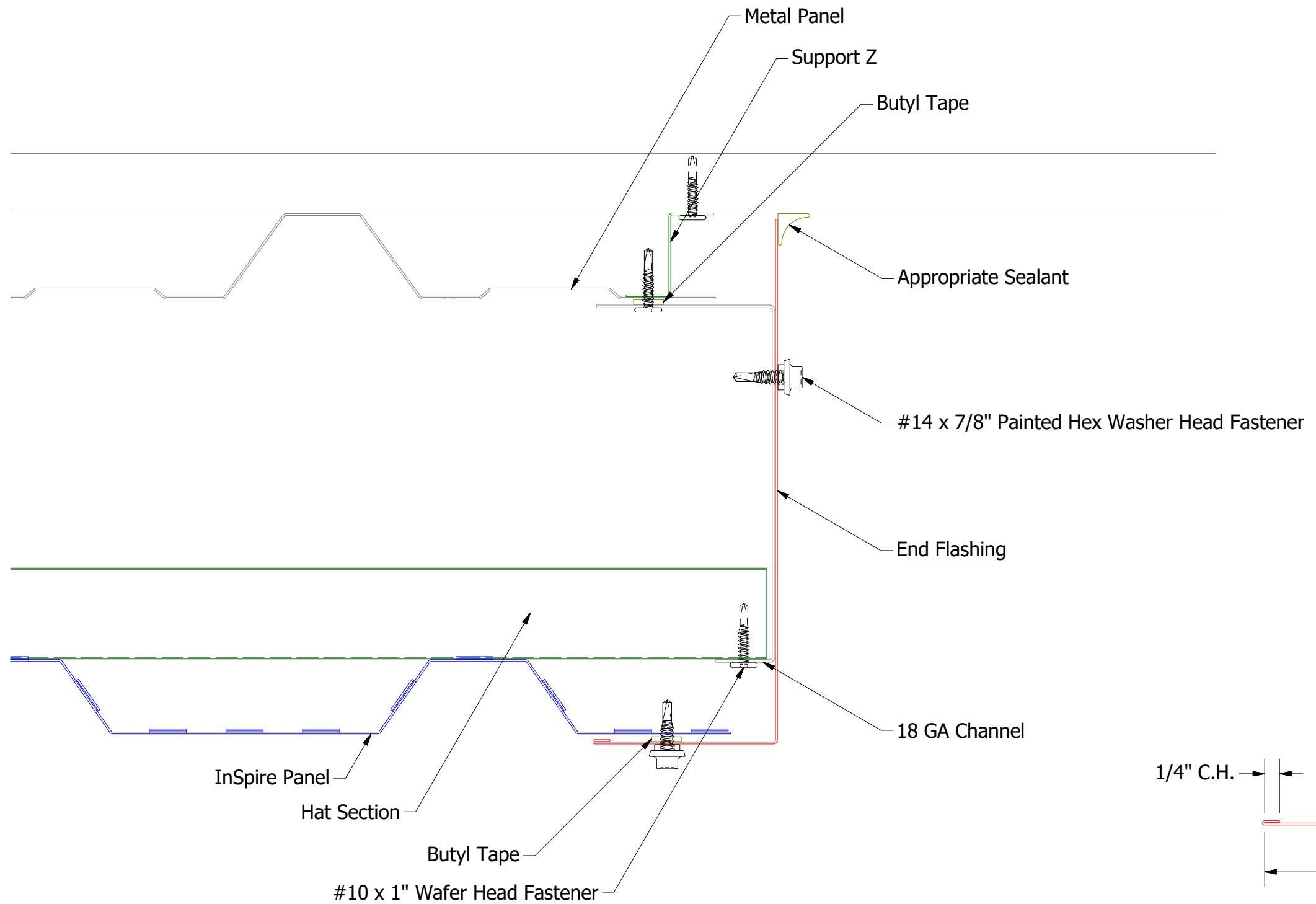
End Flashing
