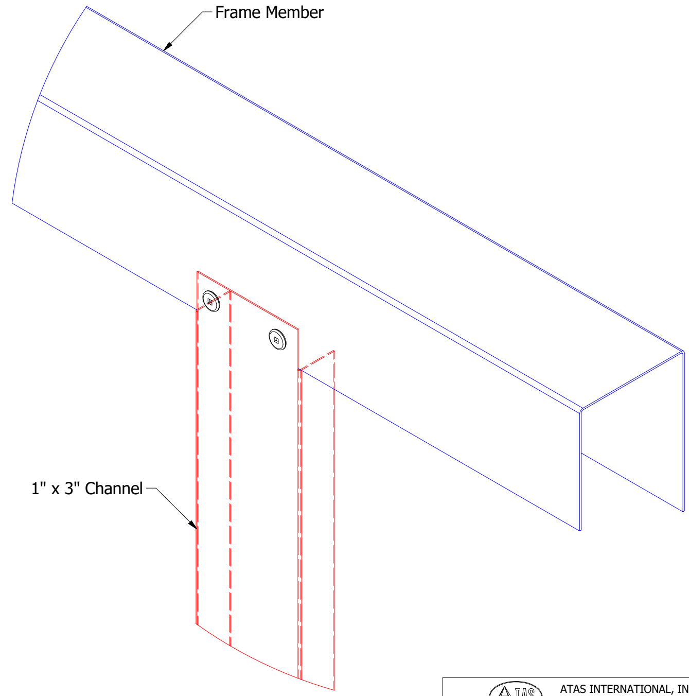
Detail A
